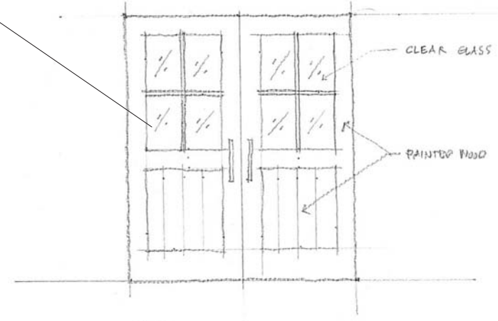
NEW SCHOOL ENTRY DOORS \frac{1}{2}'' = 1'-0'' NEW FRONT DOORS SIMILAR TO EXISTING WOOD + GLASS DOORS
